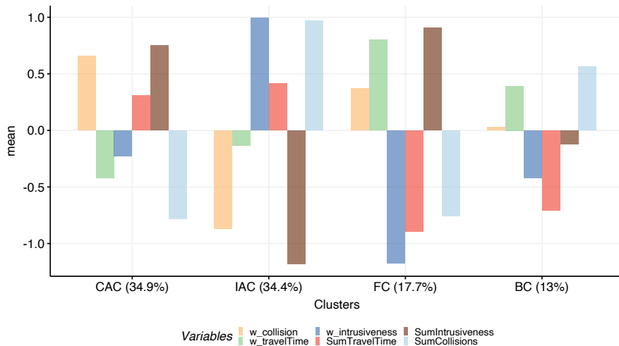
Figure 7: Bar plot of the cluster means for our robot mission planning scenario
