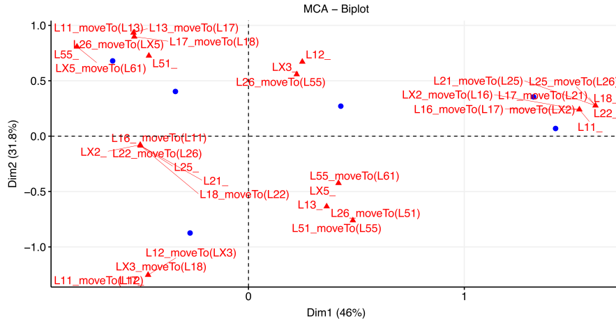
Figure 5: MCA biplot for our robot mission planning scenario. Samples are plotted as blue points and categorical variables are shown as red triangles.
