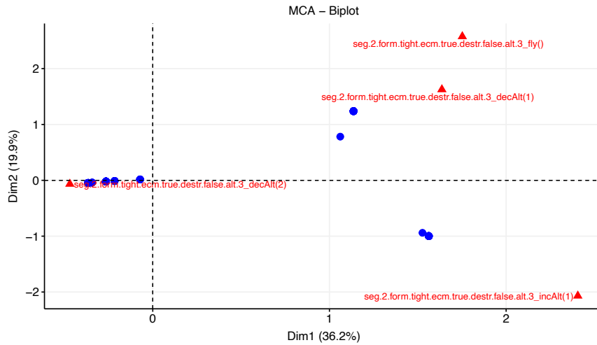
Figure 11: MCA biplot for DARTSim. Samples are plotted as blue points and categorical variables are shown as red triangles.
