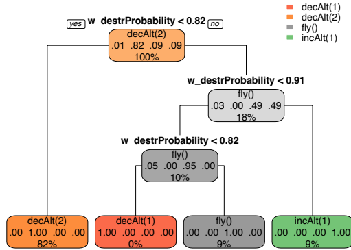
Figure 15: Decision tree plot for DARTSim (showing the selected decision in the state seg.2.form.tight.ecm.true.destr.false.alt.3 )
