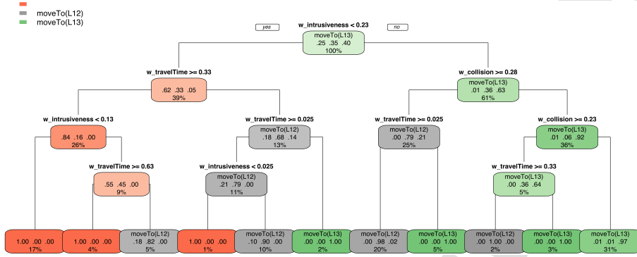
Figure 9: Decision tree plot for the robot mission planning example (showing the selected decision in the state L11)
