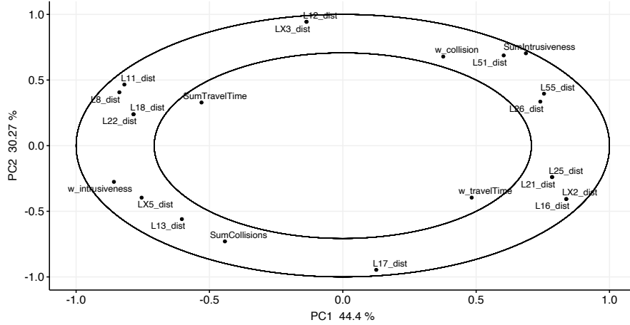
Figure 4: PCA correlation loading plot for our robot mission planning scenario
