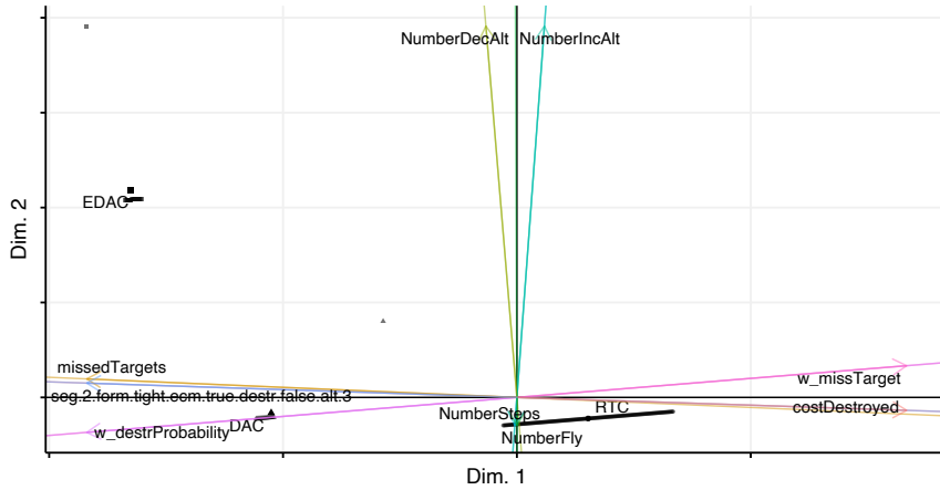
Figure 12: A reduced k-means biplot of policies (points) and quantitative variables (axes with respect to Dimensions 1 and 2) of DARTSim. The clusters are indicated as RTC, DAC, and EDAC.
