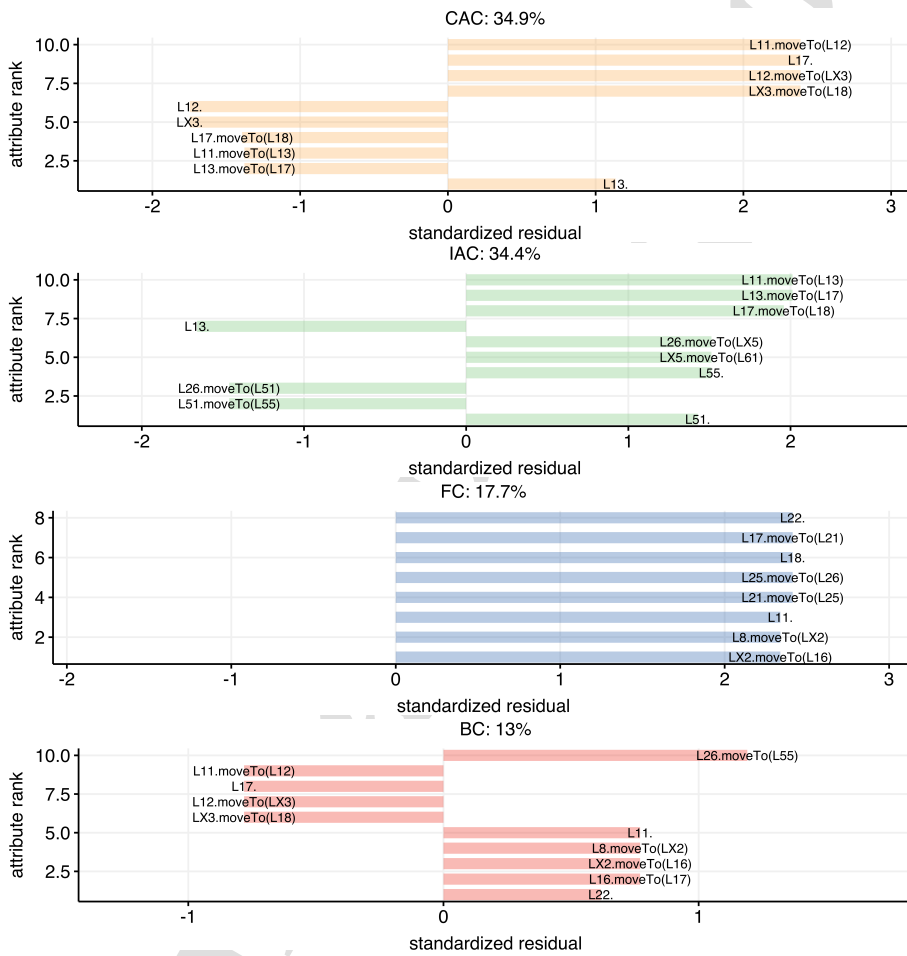
Figure 8: Variables with the highest standardized residuals (positive or negative) for each cluster in the robot mission planning scenario
