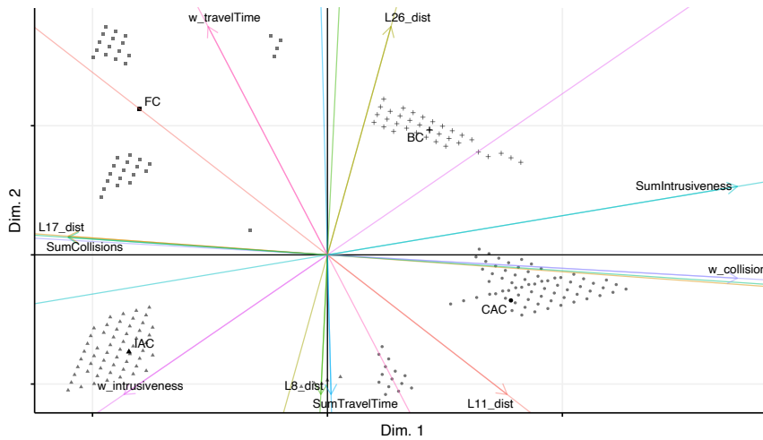
Figure 6: A reduced k-means biplot of policies (points) and quantitative variables (axes with respect to Dimensions 1 and 2). The clusters are indicated as CAC, IAC, FC, and BC.
