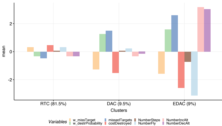
Figure 13: Bar plot of the cluster means for DARTSim
