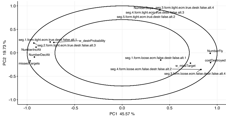
Figure 10: PCA correlation loading plot for DARTSim (all variables)
