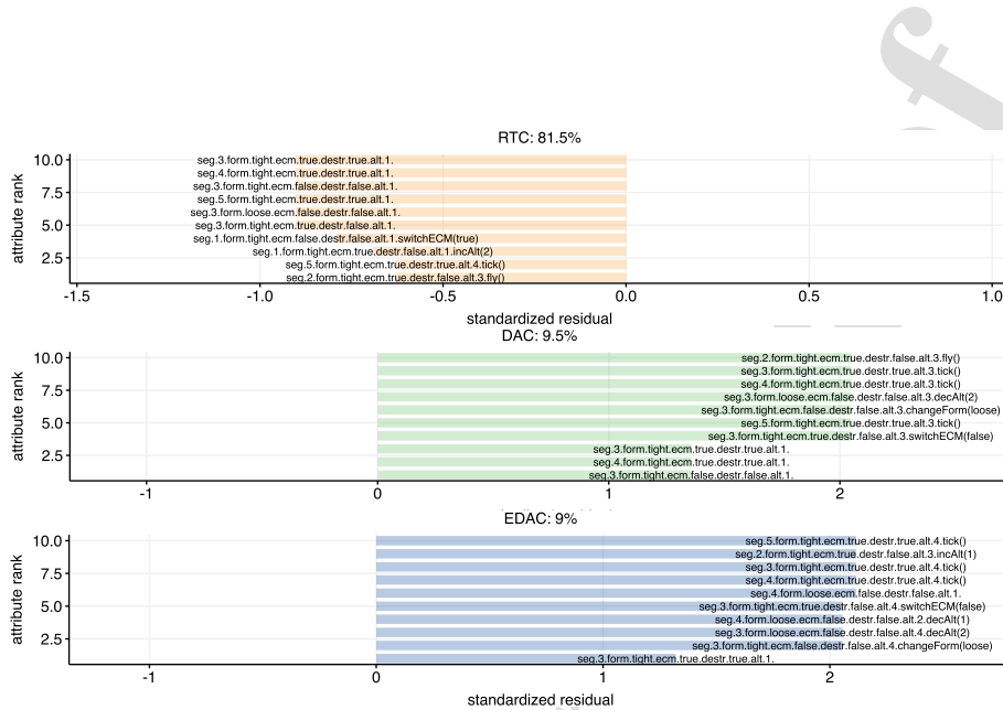
Figure 14: Variables with the highest standardized residuals (positive or negative) for each cluster in DARTSim
