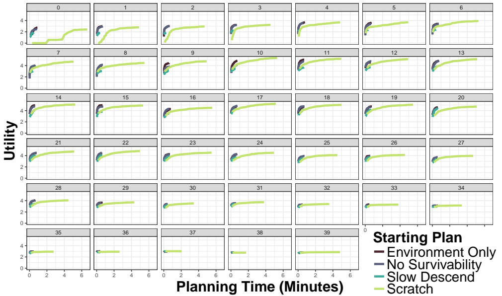
Fig. 12. Utility versus runtime by timestep.
