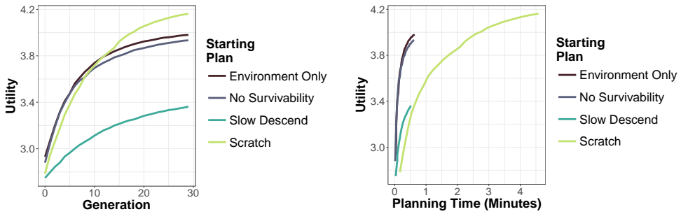
Fig. 13. Left: Utility versus generation. Right: Utility versus planning time
