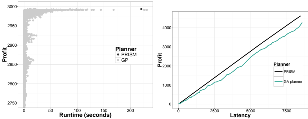
Fig. 5. Left: Profit versus planning time for GP parameter configurations. Many configurations produce similar profit results to PRISM, significantly faster. Right: Pareto fronts for profit and latency from both planners.
