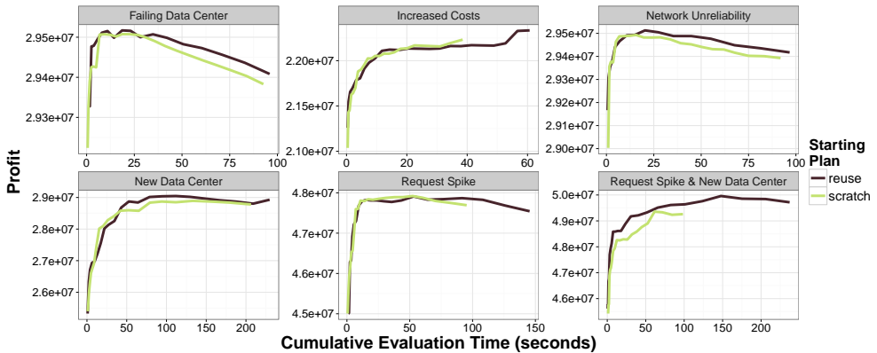
Fig. 7. Profit versus cumulative runtime for all six scenarios.
