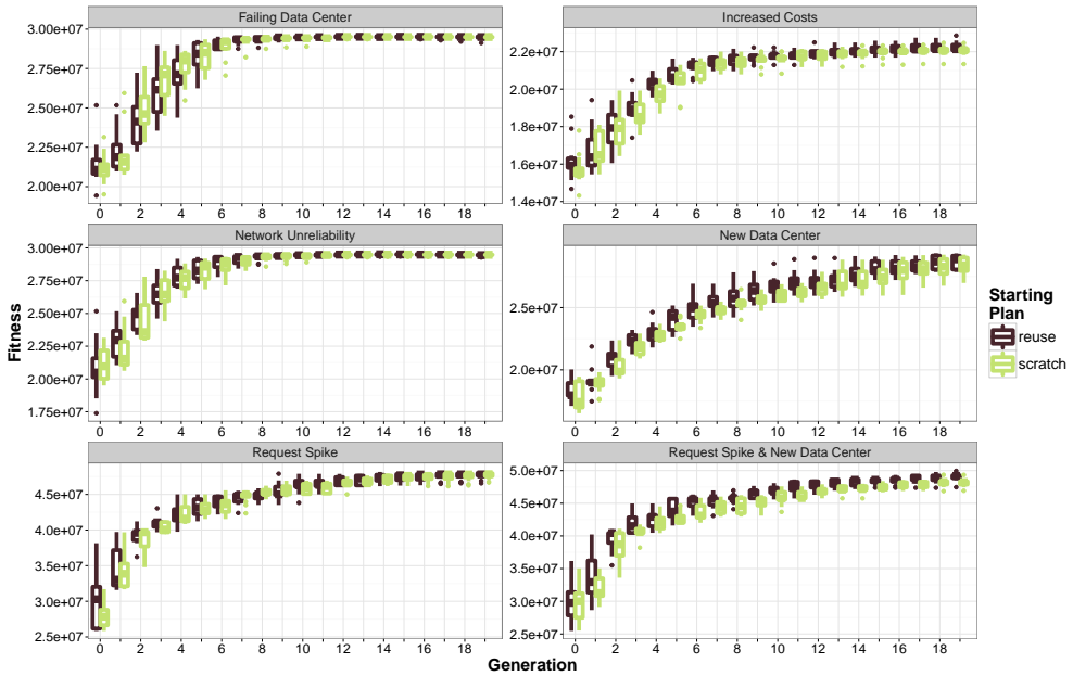
Fig. 6. Profit versus generation for all six scenarios.
